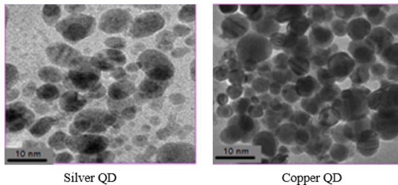
Figure 3: TEM micrograph showing spherical morphology and nanoscale distribution of synthesized quantum dots (representative image).
