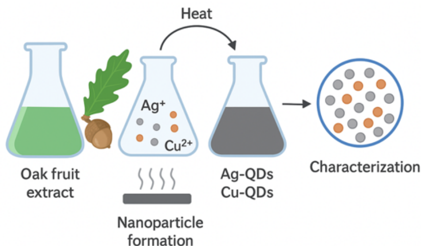
Figure 1: Schematic representation of the green synthesis process of silver (Ag-QDs) and copper (Cu-QDs) quantum dots using oak fruit extract. The extract acts as both reducing and stabilizing agent, leading to nanoparticle formation confirmed by color change and subsequent characterization.
